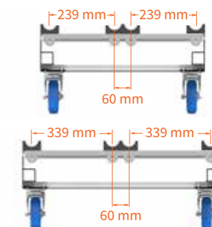
Centre-to-centre distance.
