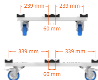
Centre-to-centre distance.
