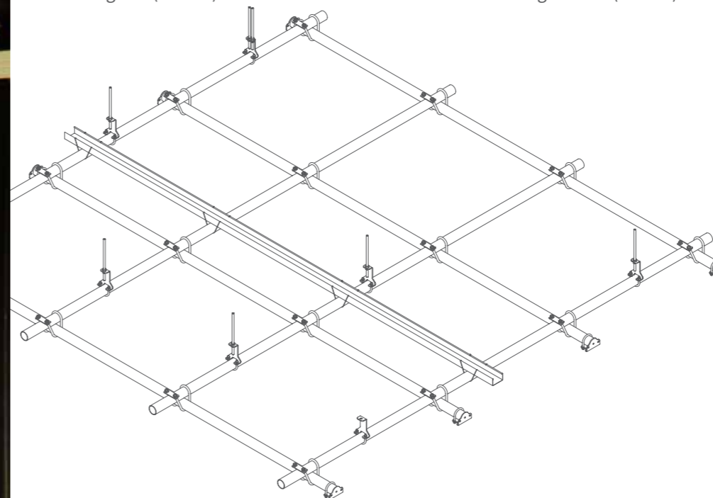
Grid Connector For two tubes of 90 degrees (50 mm).
